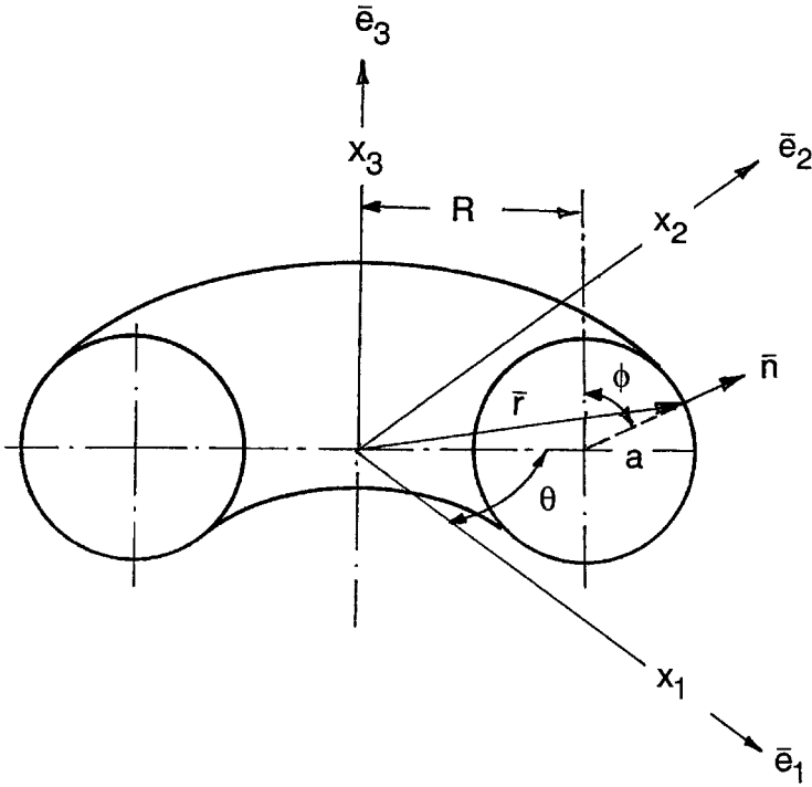
FIG. 12 The toroidal shell.
