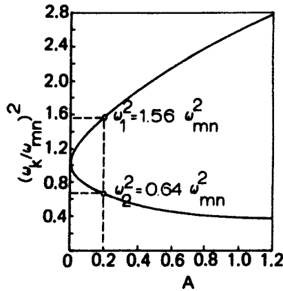
FIG. 10 Splitting of the shell natural frequencies as function of the dynamic absorber mass.
