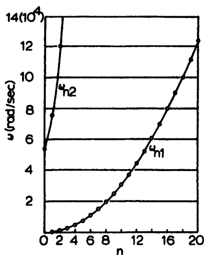
FIG. 4 Natural frequencies of a ring.
