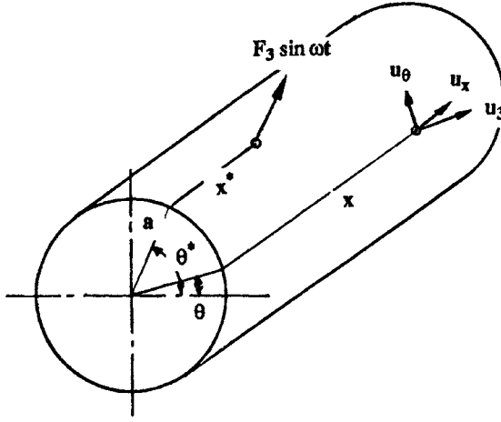
FIG. 14 Circular cylindrical shell acted on by a point force.
