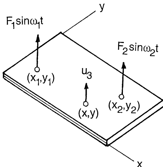
FIG. 18 Steady state forcing of a rectangular plate that will produce beating.
