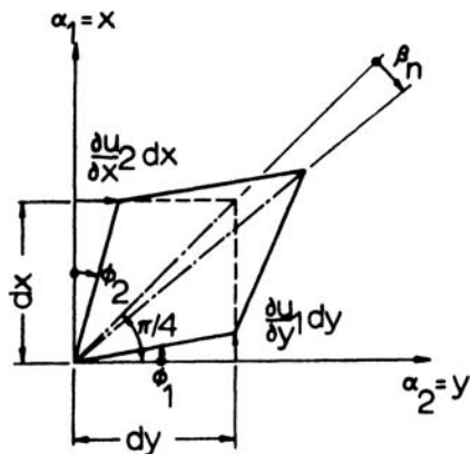
FIG. 2 Twist of an element of a rectangular plate.
