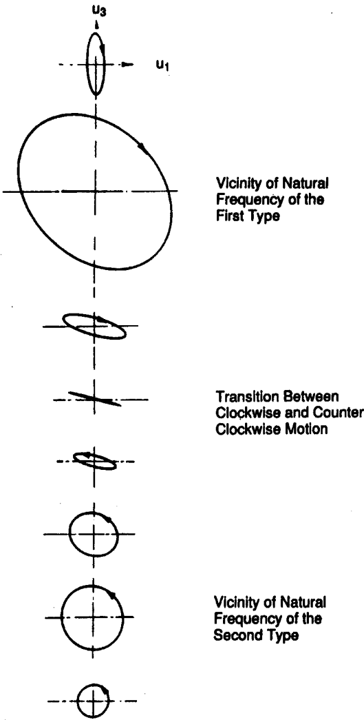
FIG. 3 Transitions of the forced response of a rotating string.
