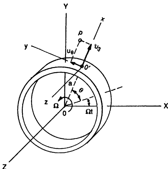
FIG. 4 Rotating ring.
