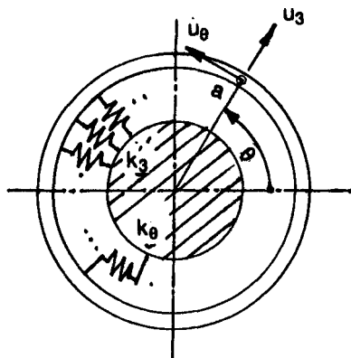
FIG. 1 Ring on an elastic foundation.
