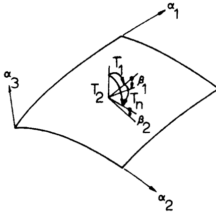
FIG. 1 Moments per unit area acting on the reference surface of a shell.
