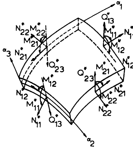
FIG. 10 Boundary force and moment resultants.
