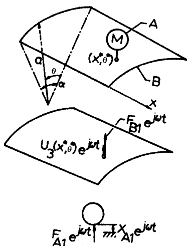
FIG. 2 Point mass connected transversely to a cylindrical panel.
