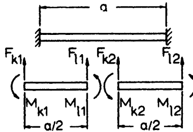
FIG. 5 Illustrative example of a transversely vibrating, clamped-clamped beam described by only two finite elements.
