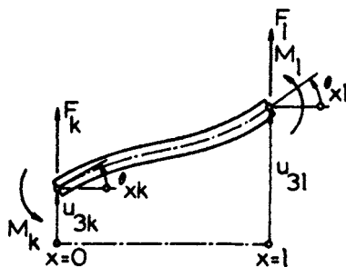
FIG. 3 Finite element for transversely vibrating beams.
