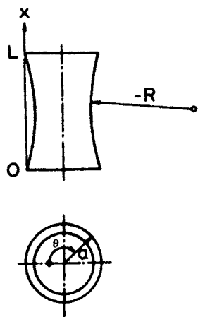
FIG. 9 Hourglass shell which is a barrel shell with negative axial curvature.
