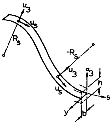
FIG. 1 Coordinate definitions for an arch.
