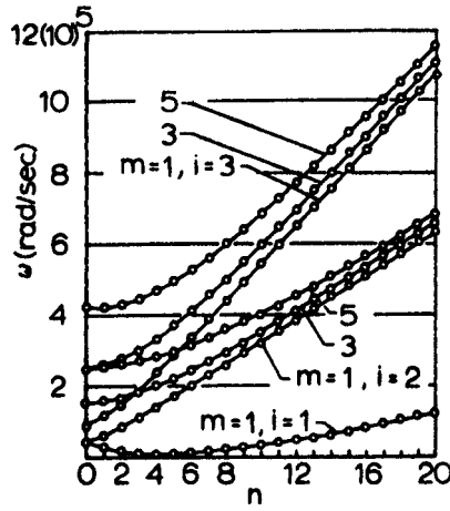
FIG. 9 Same as Fig. 8, but at a different frequency scale.
