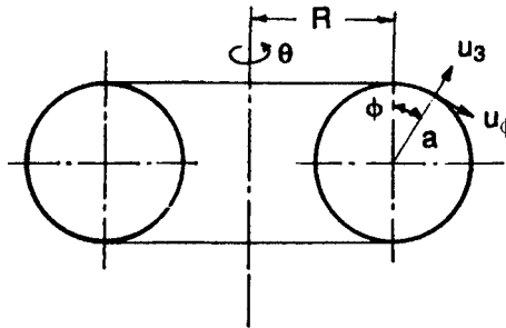
FIG. 5 Coordinate definitions for a toroidal shell.
