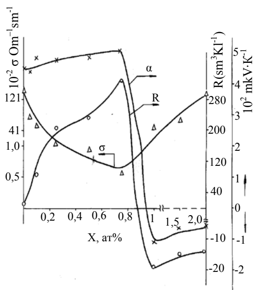
Figure1. Association of arguments on concentration of content Nd in an alloy \text{Sn}_{1-x}\text{Nd}_x\text{Se} : x - thermopower ( \alpha ); O - Hall coefficient ( R ); \Delta - An electrical conductivity ( \sigma ).
